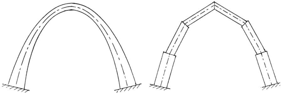
Fig. 1 Discretisation of a Non-Prismatic Arch
