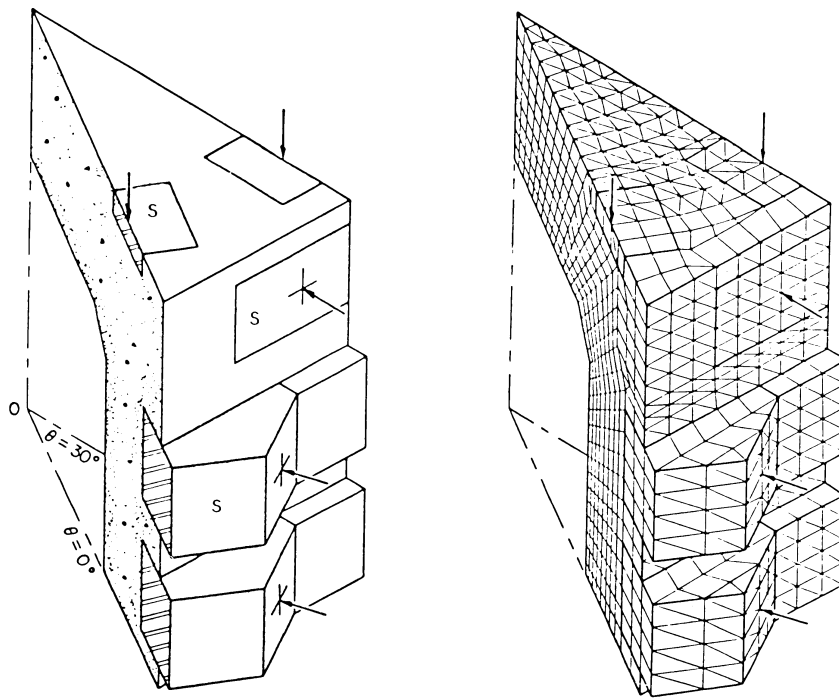
Fig. 7 Finite Element Modelling of One-Twelfth Symmetry Segment of Top Half of Prestressed Concrete Nuclear Reactor Model. (s = steel)
