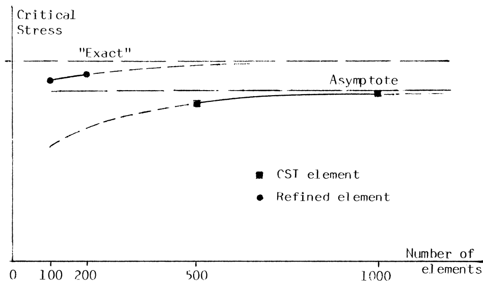
Fig. 8 Convergence Capabilities of Different Elements
