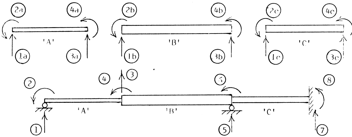
Fig. 4 Continuous Beam Assembled from Three Members
